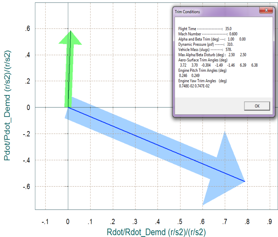
Ratios of Roll and Yaw Accelerations Over Corresp Control Acceleration Demands ( \dot{R} dot & \dot{P} dot)/ \dot{P} dot_Demand and ( \dot{R} dot & \dot{P} dot)/ \dot{R} dot_Demand, (rad/sec2) / (rad/sec2)
