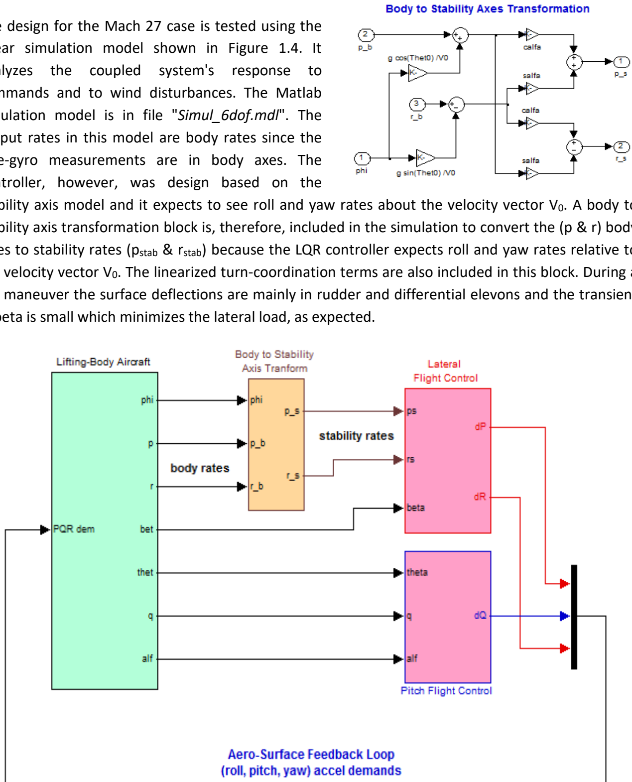
Figure 1.4a Simulation Model in File "Simul_6dof.Mdl"
