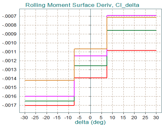
Figure 5.5 Right Elevon Aero-Surface Lateral Increments and Derivatives
