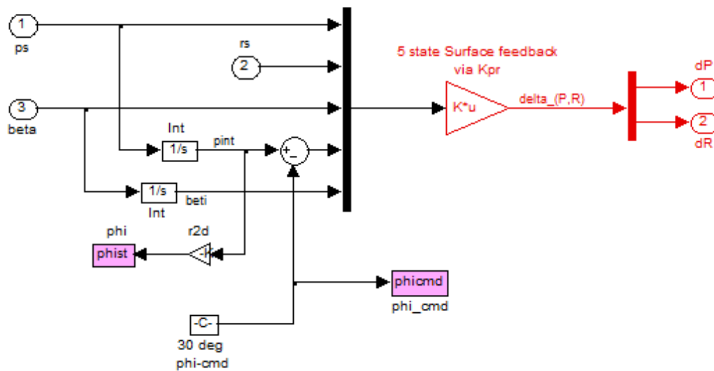
Figure 1.5 Pitch and Lateral state-feedback Control Laws derived by the LQR method
