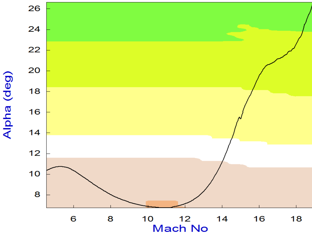
Yaw Control Effort Contour Plot (Mach vs Alpha)
