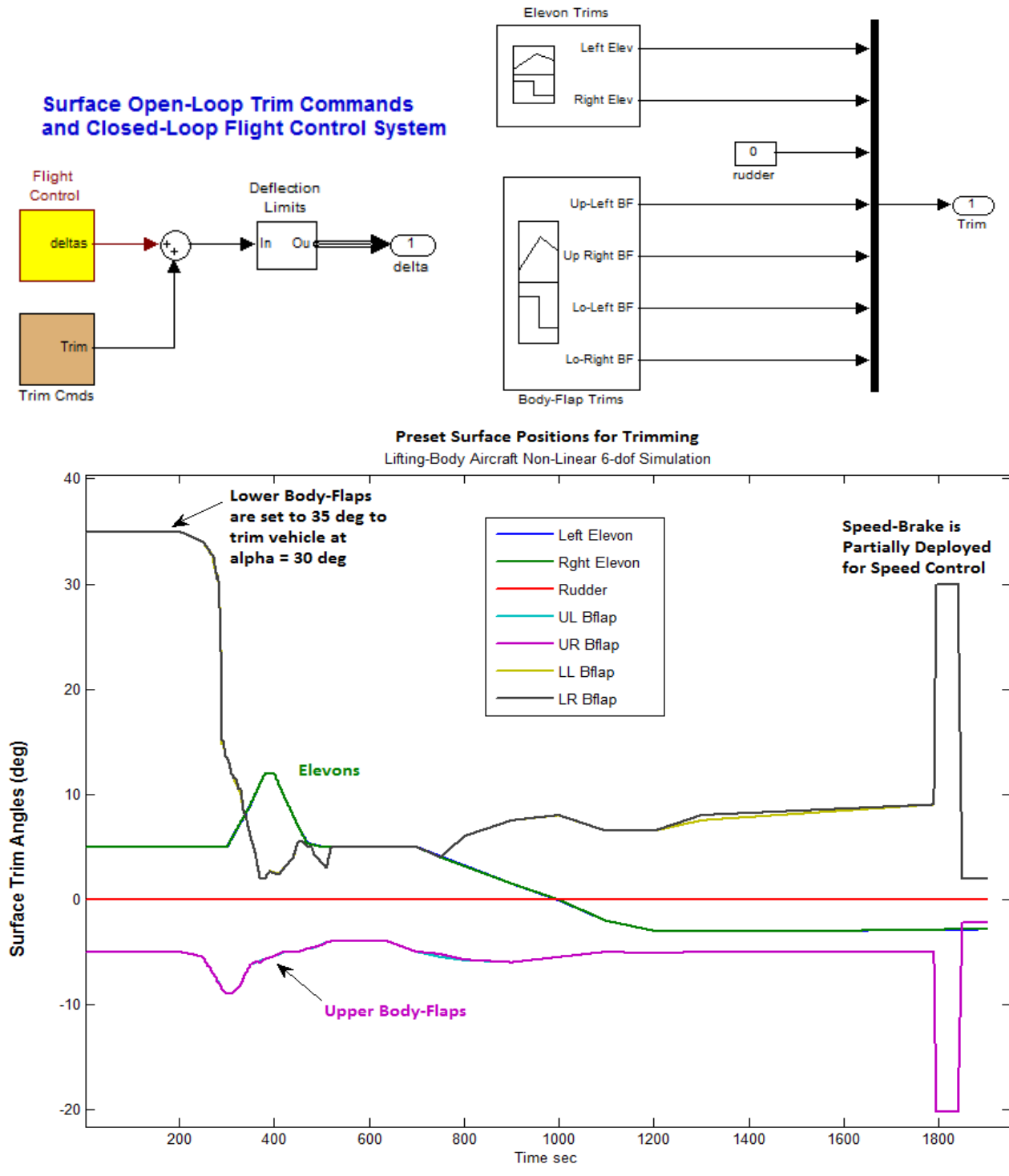
Figure 1.5.15 Aero-Surface Scheduling is based on previous Trim Analysis
