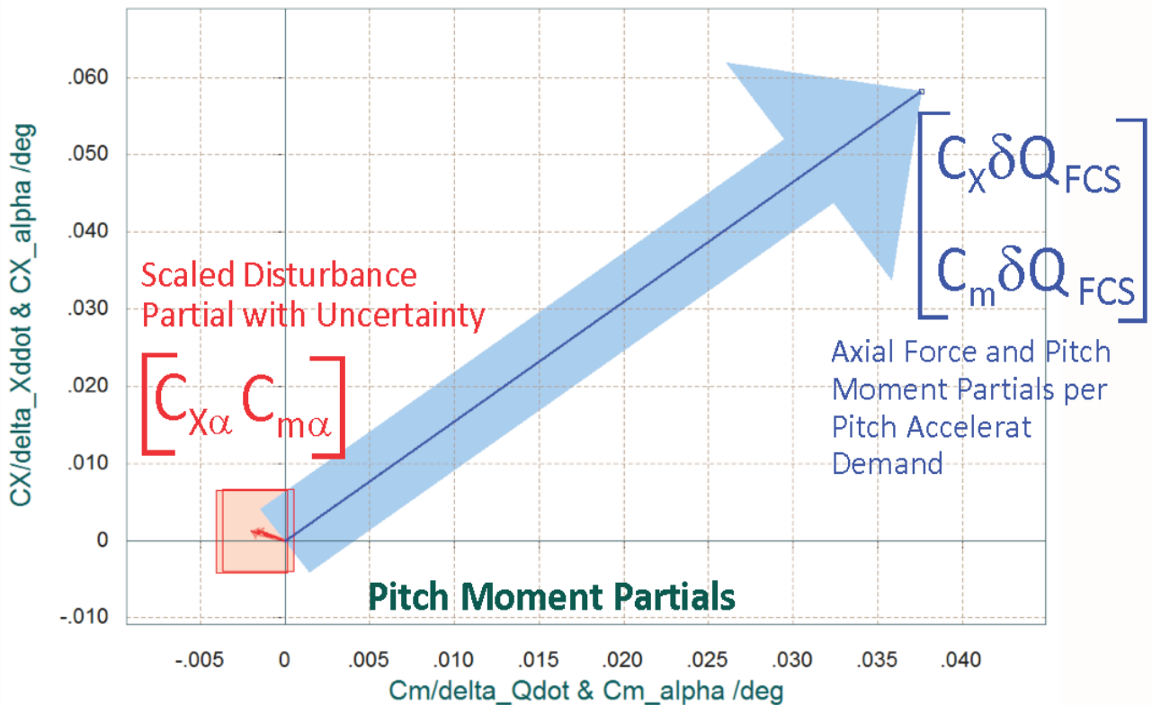
Comparison Between Control Moment & Force Partial: \{Cm/\delta Q \ \& \ CX/\delta X\} (Blue and Green), Against Partial: \{Cm/\alpha \ \& \ CX/\alpha\} (Red Vectors)
